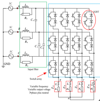
Fig.1 Topology of 3X4MC.
