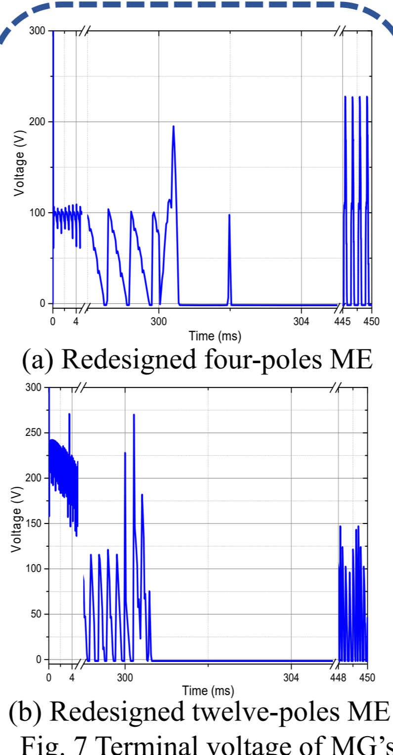
Fig. 7 Terminal voltage of MG's field winding
